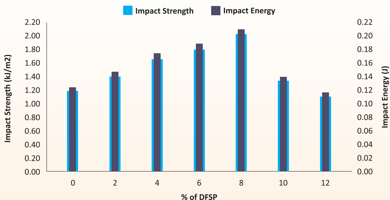
Figure 3: Effect of varied wt% of DFSP on impact strength and impact energy
